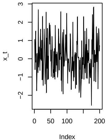
ARMA(1,1) weakARMA
