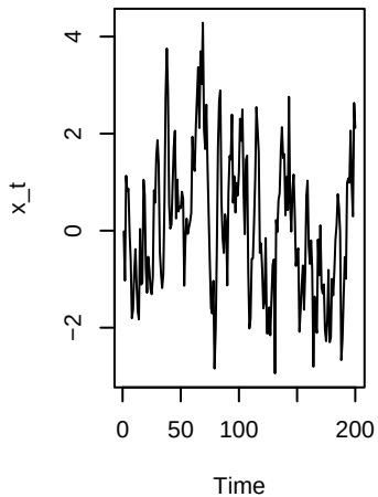
AR(1) arima.sim
