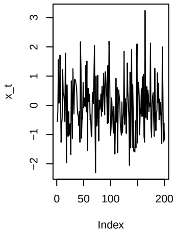
AR(1) weakARMA
