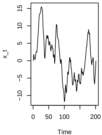
ARIMA(1,1,0) arima.sim
