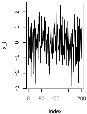
MA(2) weakARMA
