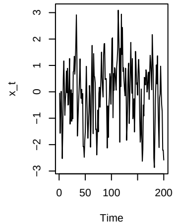
MA(2) arima.sim
