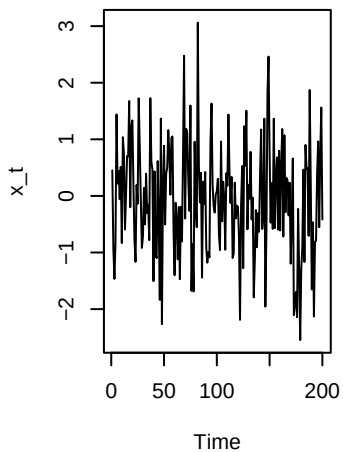
ARMA(1,1) arima.sim
